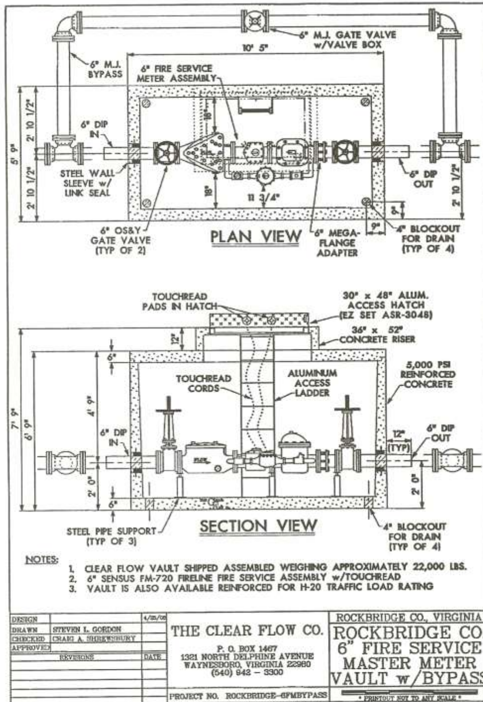
Figure 31-Fire Line Meter Vault-6" Meter
