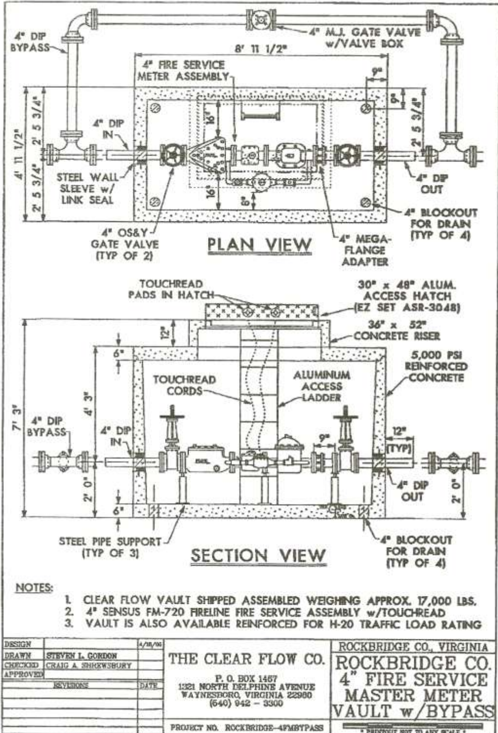
Figure 30. Fire Line Meter Vault-4" Meter
