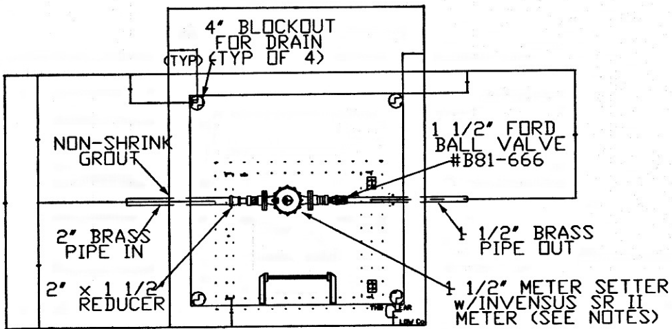
PLAN VIEW
