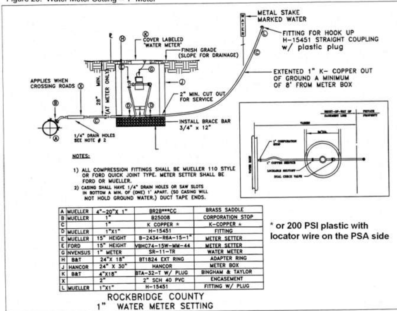
Figure 25. Water Meter Setting -- 1" Meter
