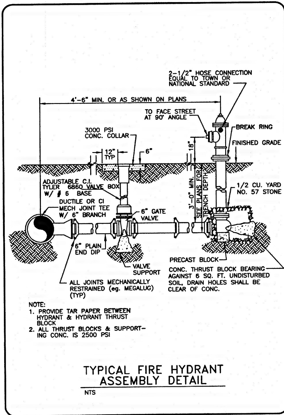
Figure 21. Fire Hydrant Assembly Detail
