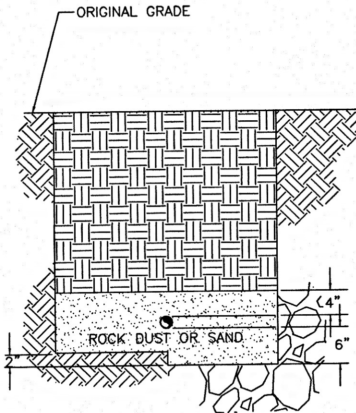
SMALL PIPE BEDDING DETAIL -FOR 3/4" TO 2" PIPE-
