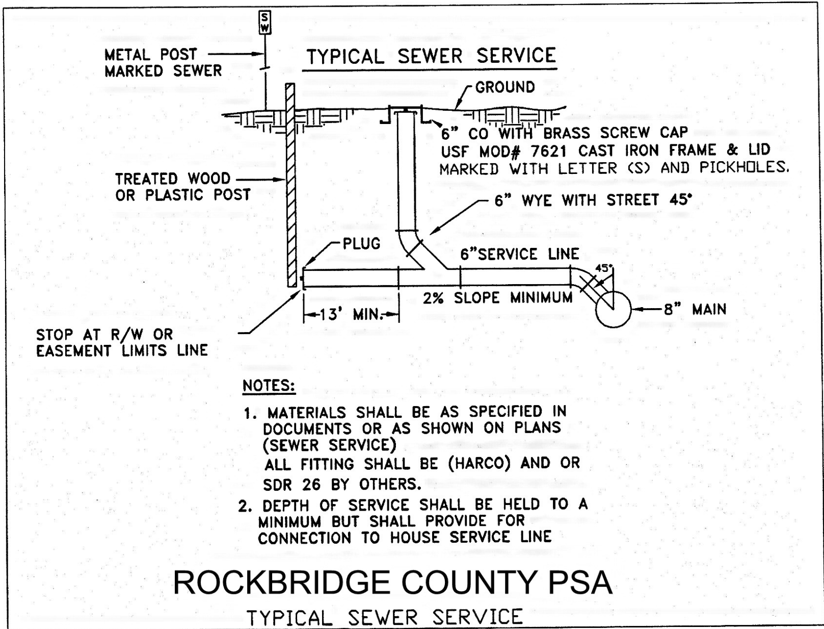
Figure 17. Typical Sewer Service
