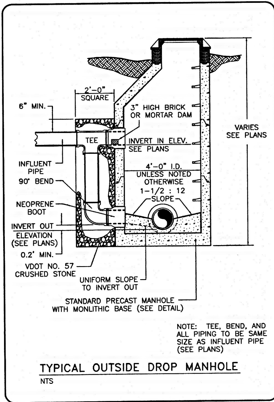
Figure 13. Typical Outside Drop Manhole
