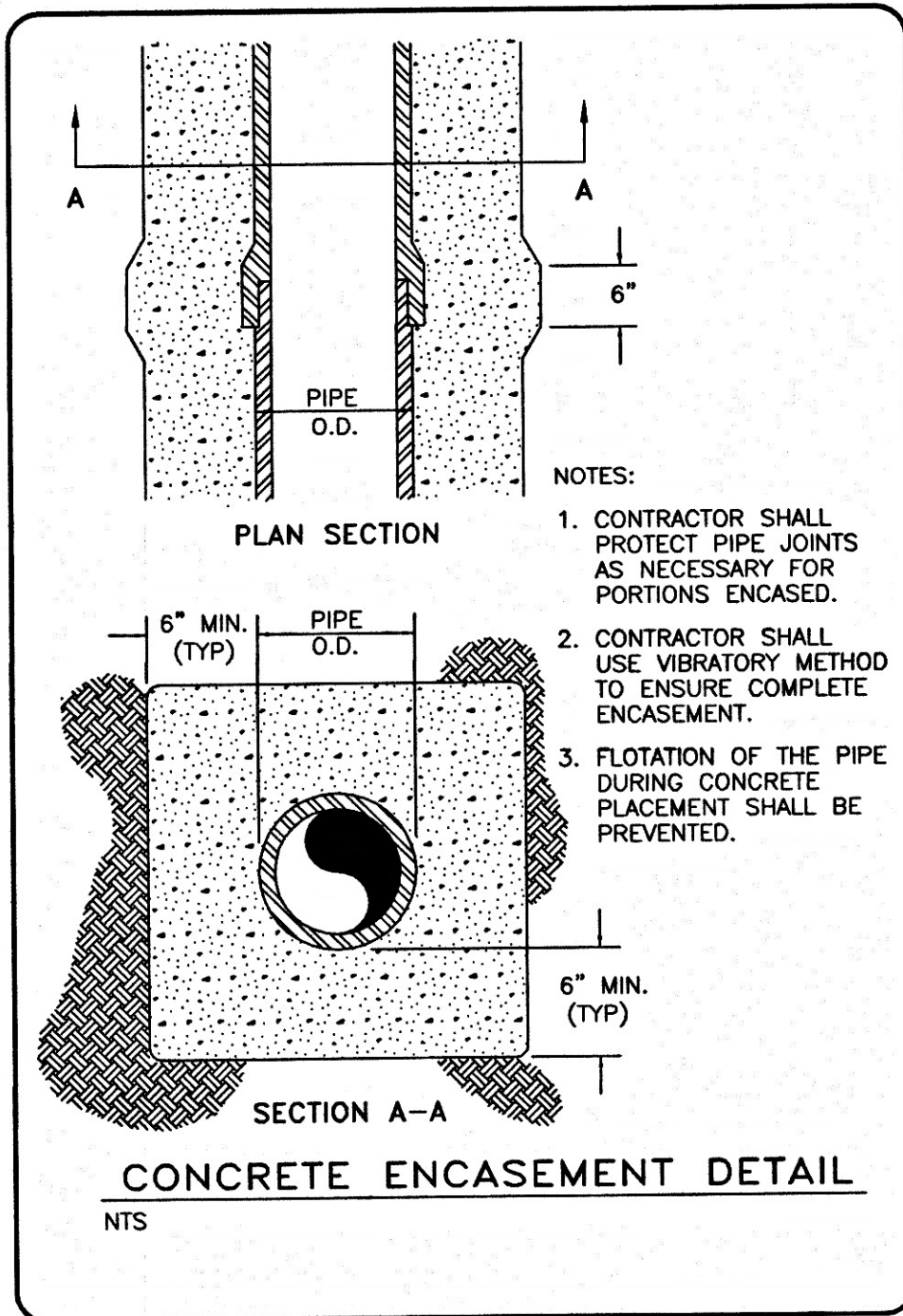
Figure 6. Concrete Encasement Detail
